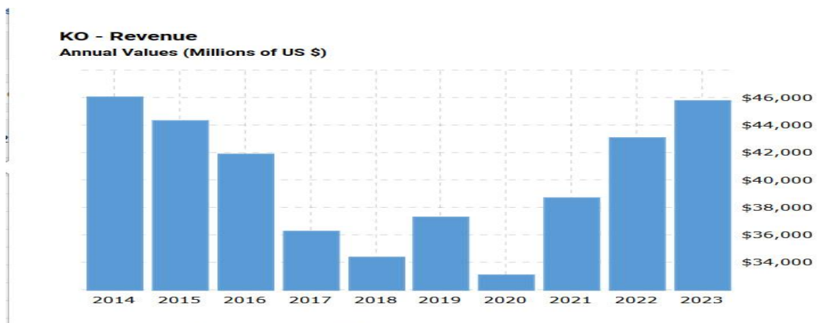
Graph 4. Benchmark Analysis:
